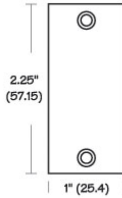
BLANK LATCH FRONT
